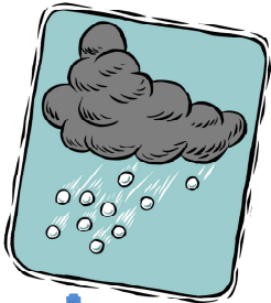
hail
