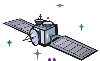
satellite
