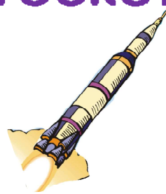
rocket
