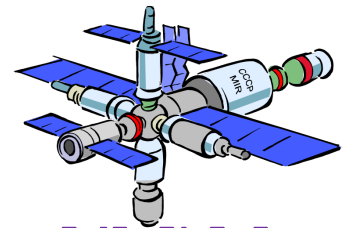
space station
